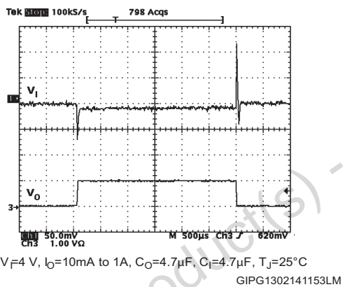
Figure 22. Load transient
