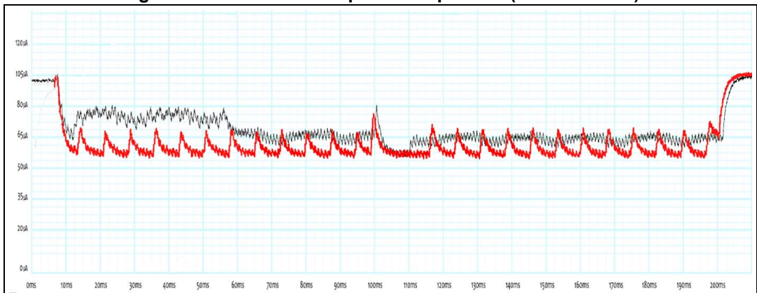
Figure 23. Power consumption comparison (FIFO ON/OFF)
