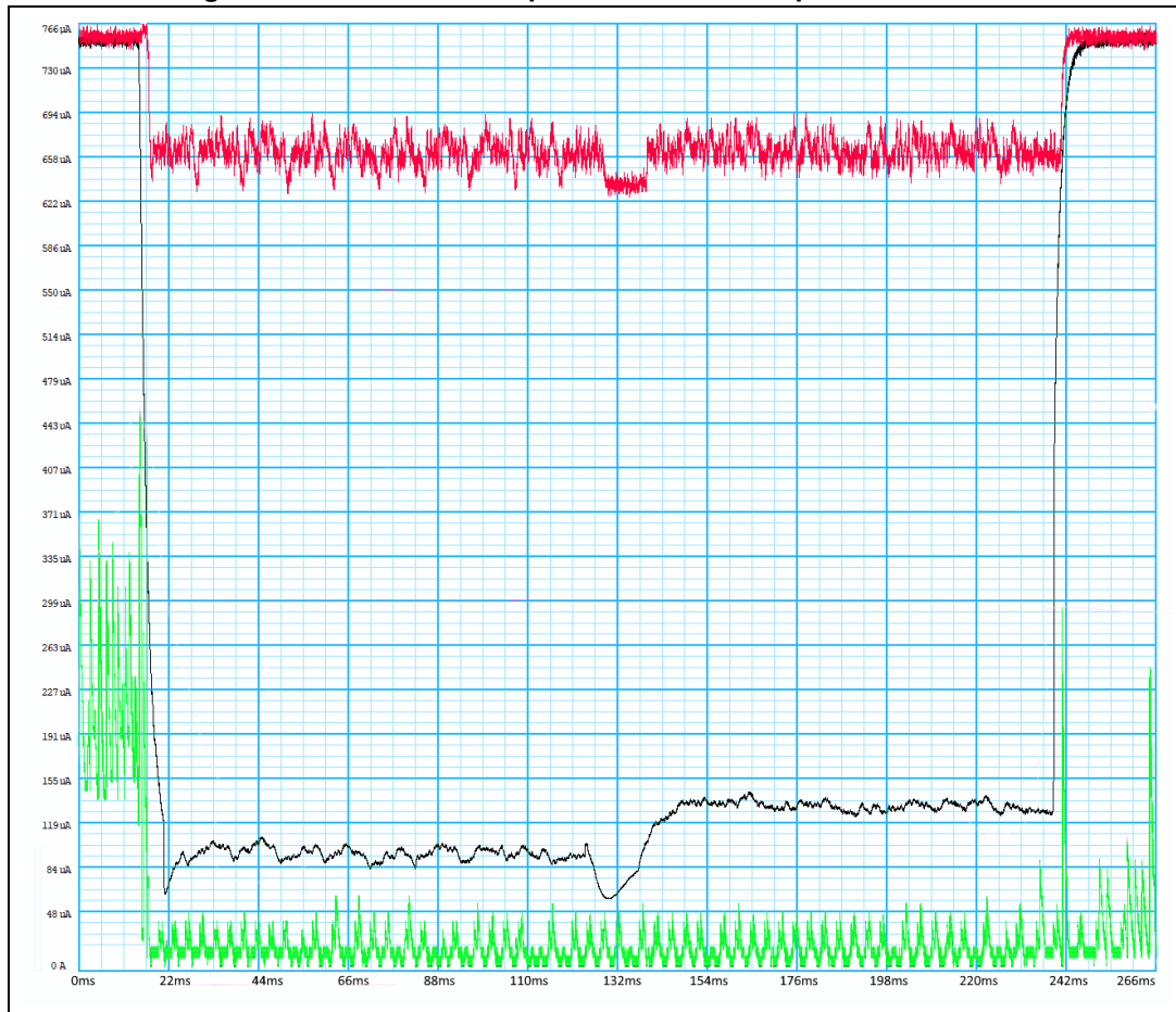
Figure 22. Power consumption for different operation modes
