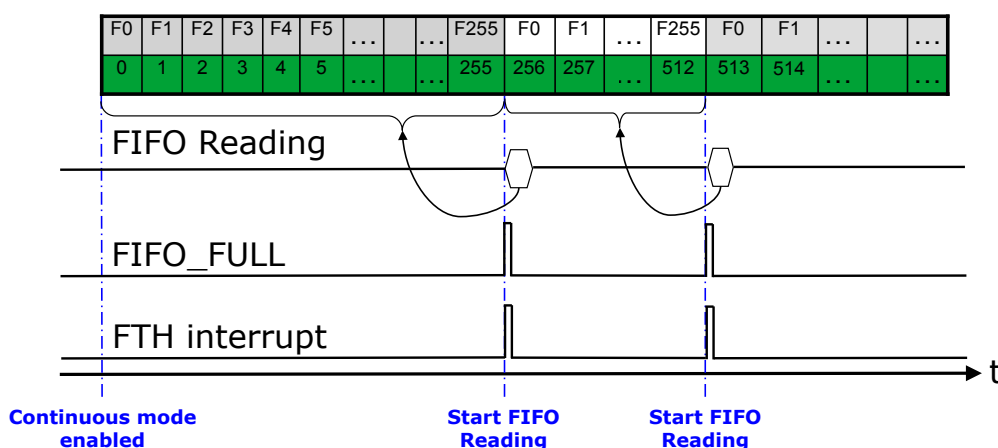
Figure 14. Continuous mode with interrupt trigger
