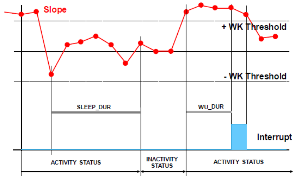
Figure 11. Activity/Inactivity recognition
