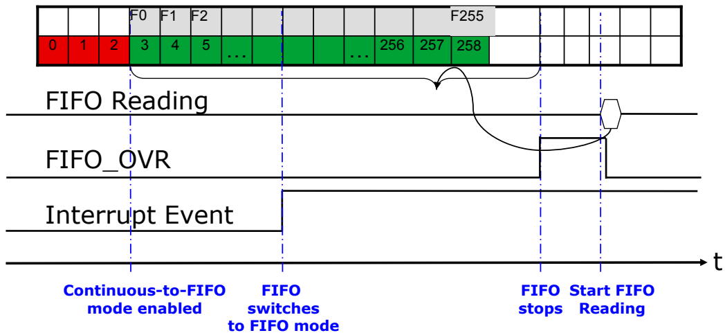
Figure 15. Continuous-to-FIFO mode: interrupt latched and nonlatched
