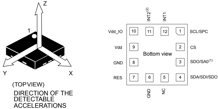
Figure 1. Pin connections
