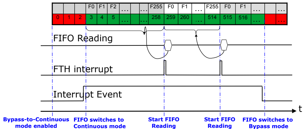
Figure 16. Bypass-to-continuous mode
