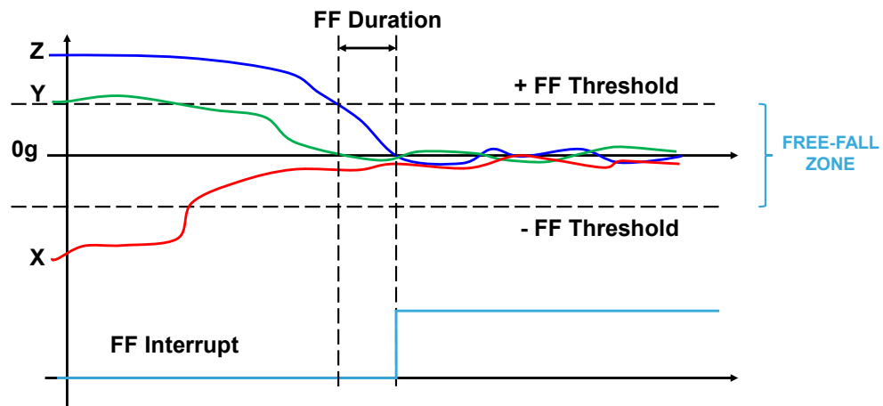
Figure 5. Free-fall interrupt
