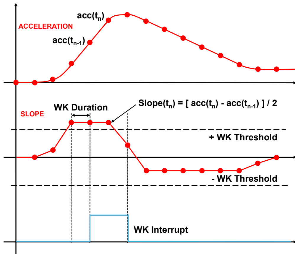
Figure 6. Wake-up interrupt
