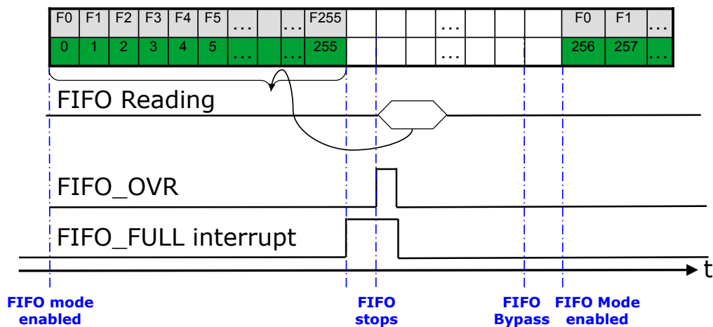
Figure 13. FIFO mode behavior
