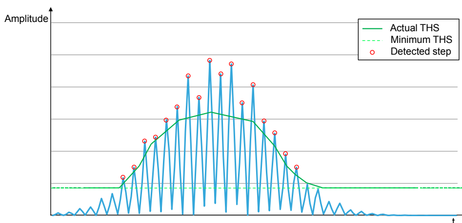
Figure 12. Minimum threshold
