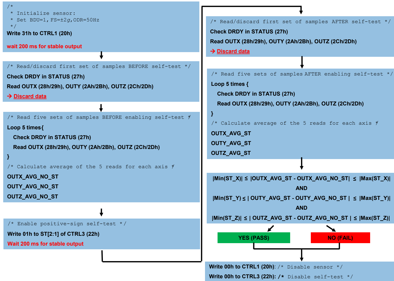
Figure 17. Accelerometer self-test procedure
