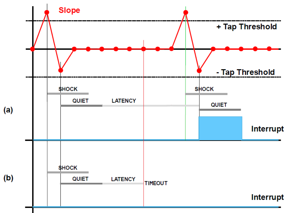
Figure 9. Double-tap event recognition (LIR bit = 0)
