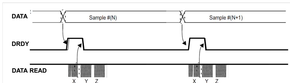
Figure 4. Data-ready signal
