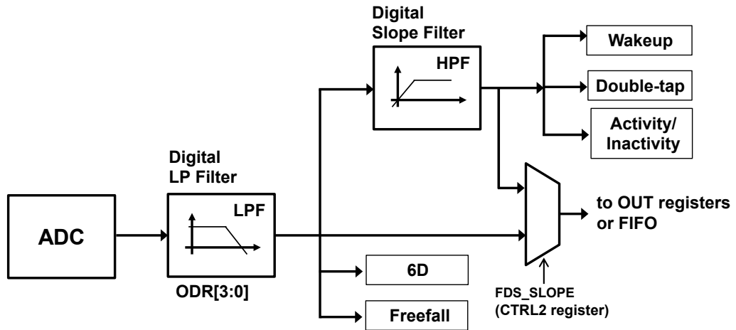
Figure 2. Accelerometer sampling chain
