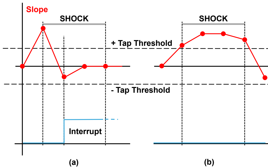
Figure 8. Single-tap event recognition
