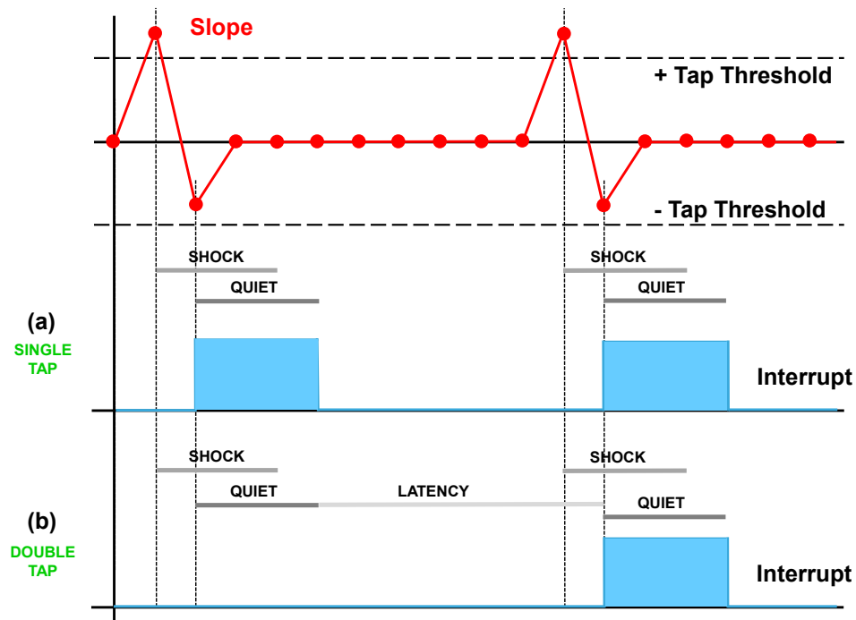
Figure 10. Single and double-tap recognition (LIR bit = 0)
