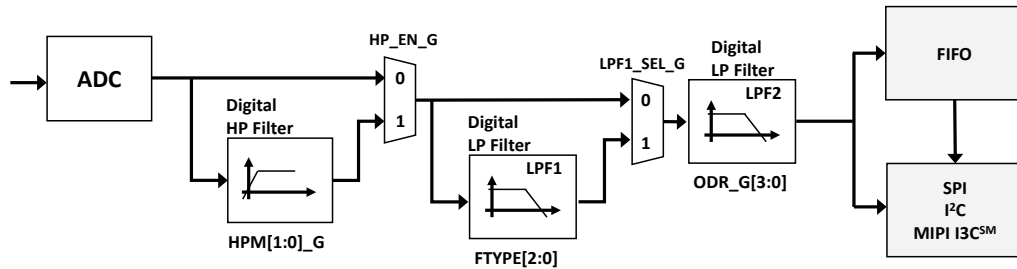
Figure 4. Gyroscope digital chain
