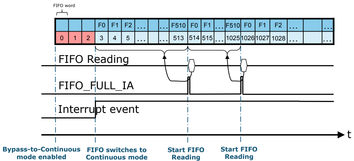
Figure 20. Bypass-to-continuous mode
