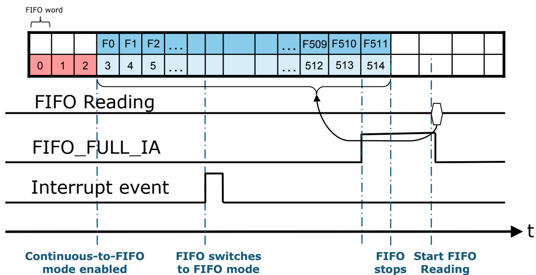
Figure 19. Continuous-to-FIFO mode
