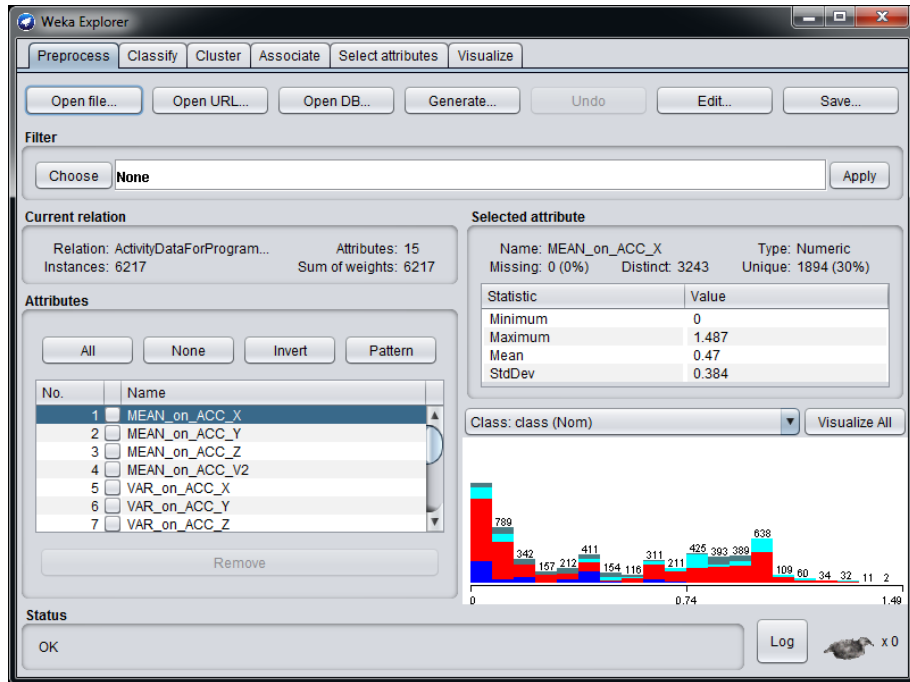
Figure 24. Weka preprocess
