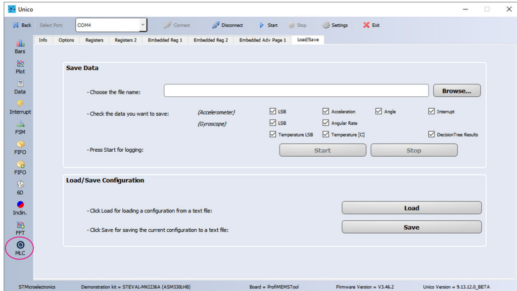
Figure 20. Unico GUI
