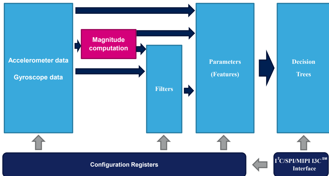
Figure 2. Machine learning core in the ASM330LHBG1
