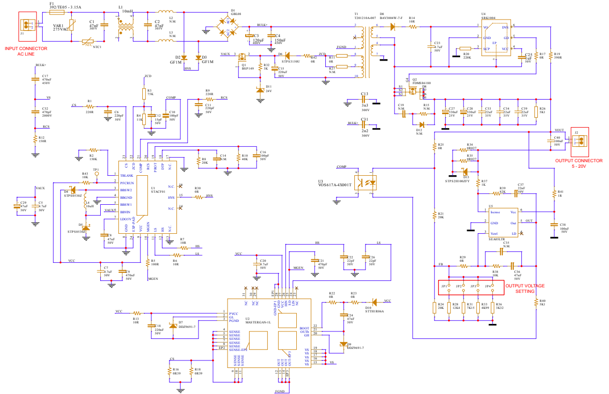
Figure 1. EVLSTACF01-65WU - schematic
