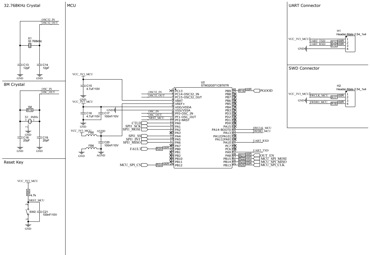
Figure 4. STEVAL-IOL8DOCB circuit schematic (3 of 4)
