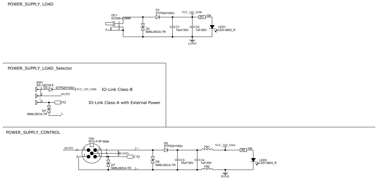
Figure 2. STEVAL-IOL8DOCB circuit schematic (1 of 4)
