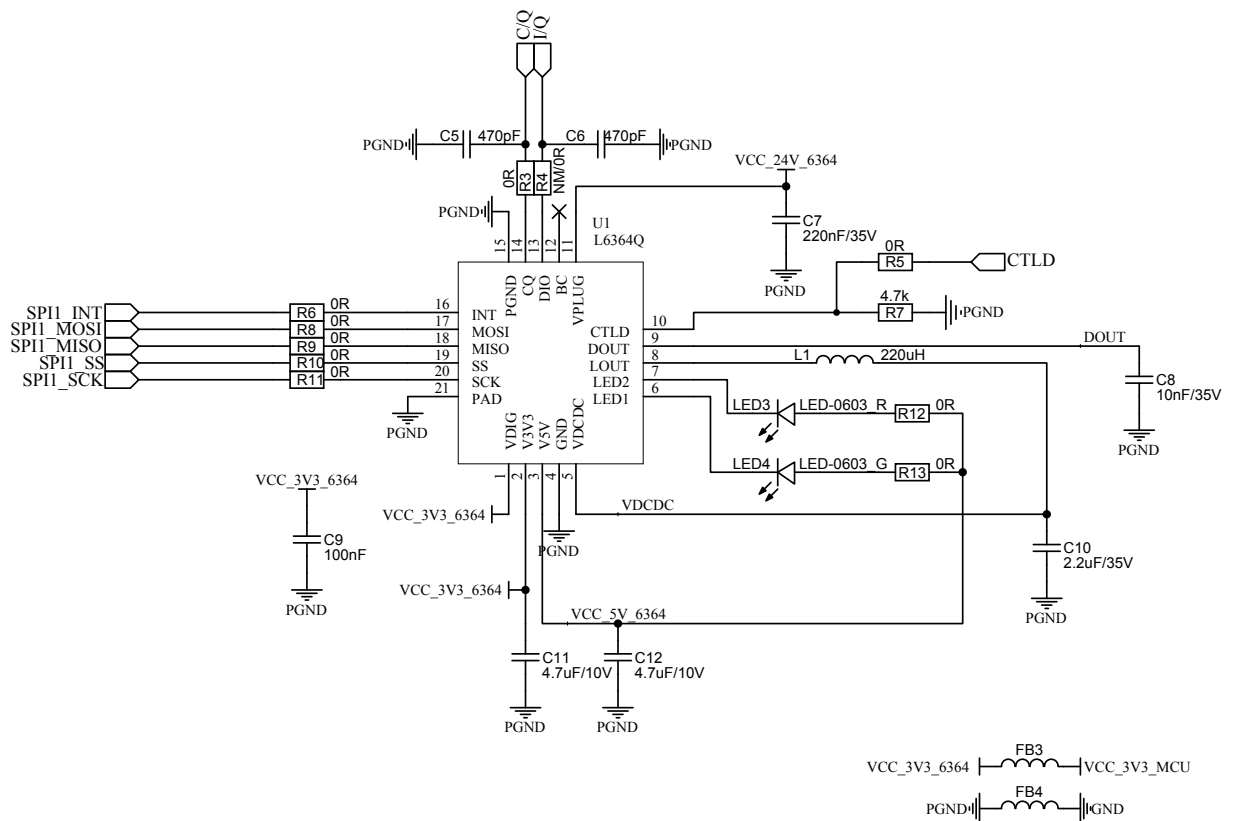
Figure 3. STEVAL-IOL8DOCB circuit schematic (2 of 4)
