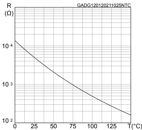
Figure 17. Typical NTC resistance vs temperature
