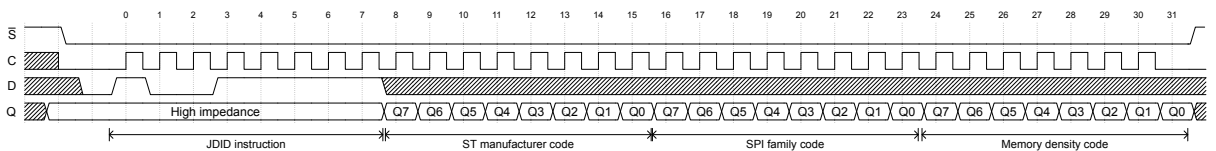
Figure 29. JEDEC identification
