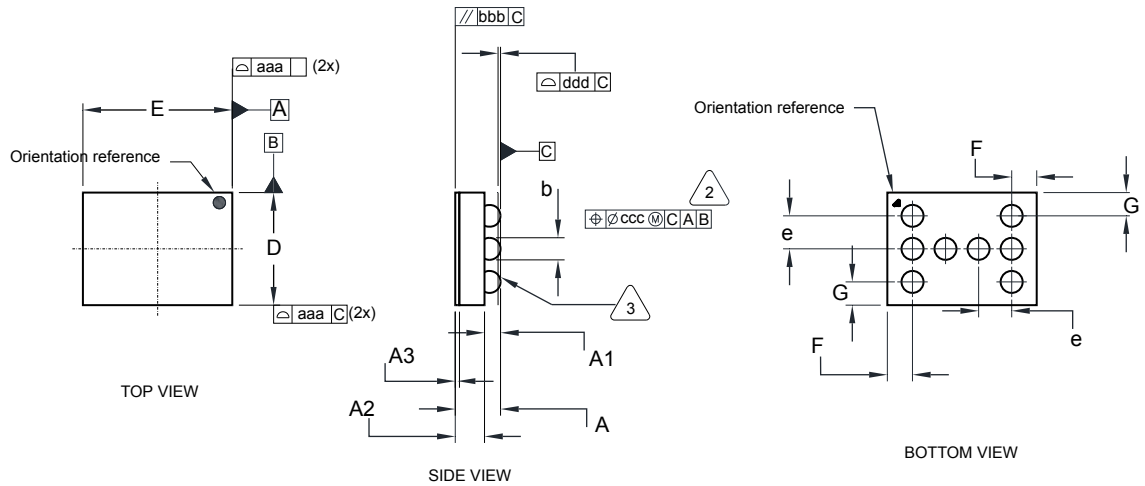
Figure 44. WLCSP8 - Outline
