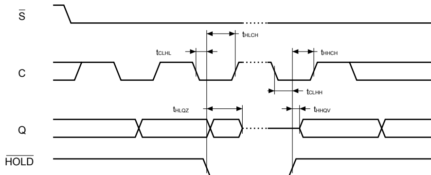
Figure 38. Hold timing
