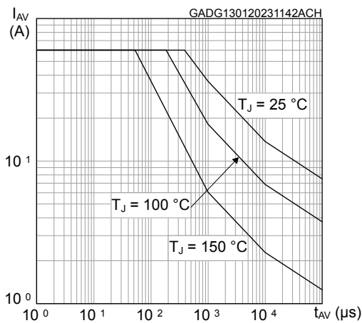
Figure 5. Avalanche characteristics
