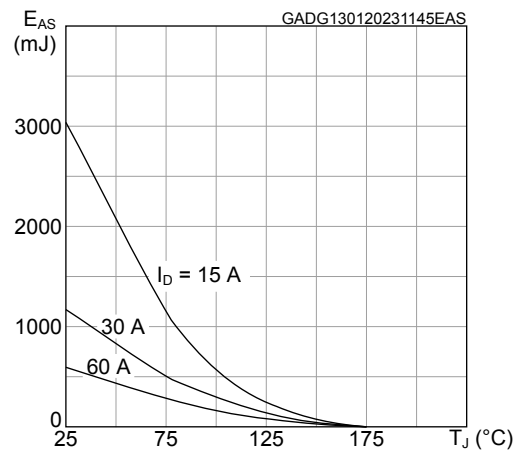
Figure 6. Avalanche energy
