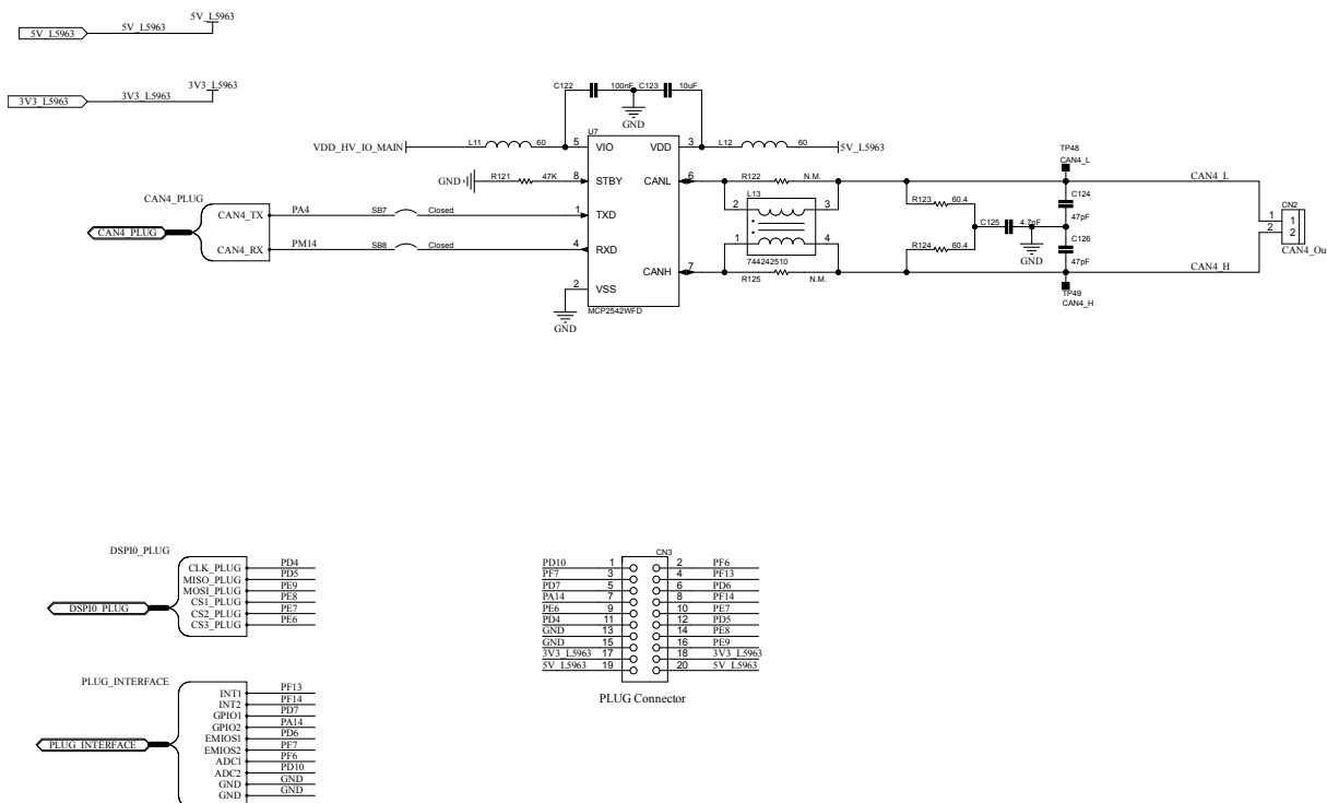
Figure 10. AEK-COM-10BASET circuit schematic (10 of 10)
