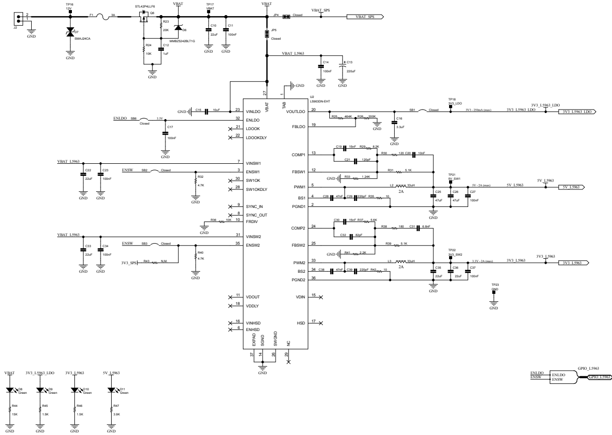
Figure 2. AEK-COM-10BASET circuit schematic (2 of 10)
