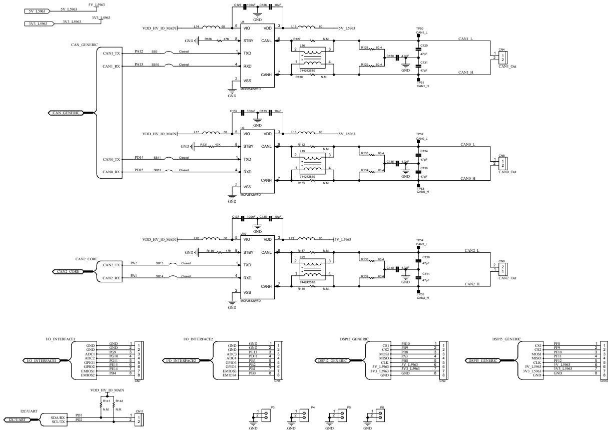
Figure 9. AEK-COM-10BASET circuit schematic (9 of 10)
