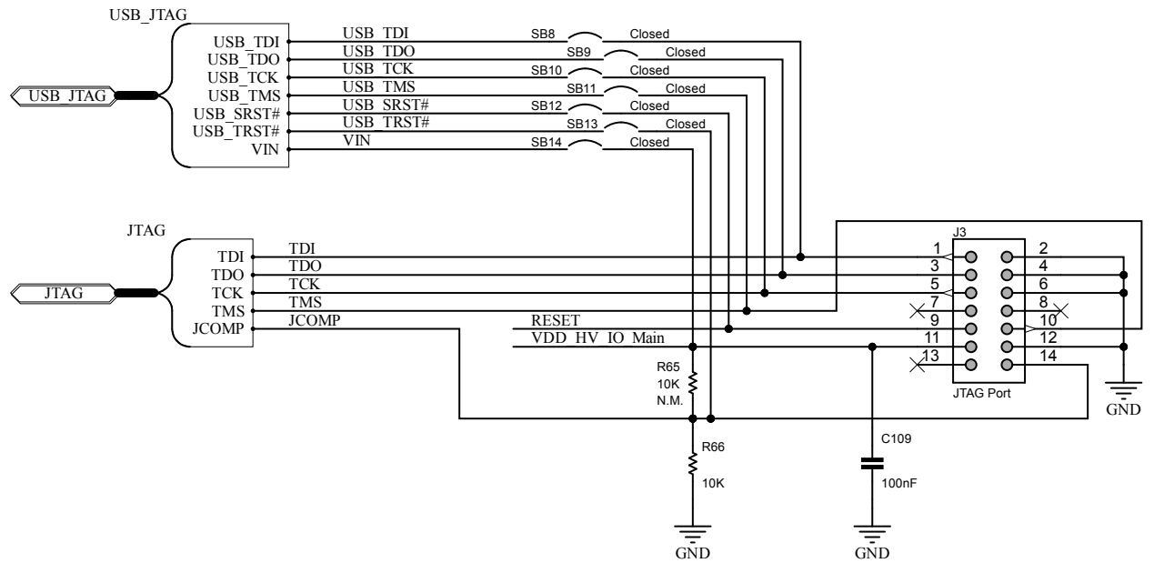
Figure 6. AEK-MCU-C4MINI1 circuit schematic (6 of 12)
