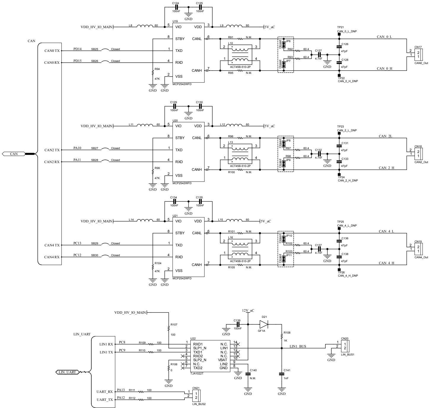
Figure 8. AEK-MCU-C4MINI1 circuit schematic (8 of 12)
