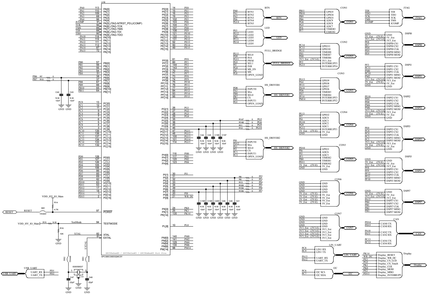
Figure 4. AEK-MCU-C4MINI1 circuit schematic (4 of 12)
