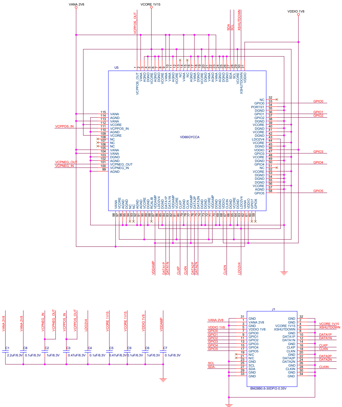
Figure 1. Circuit schematic
