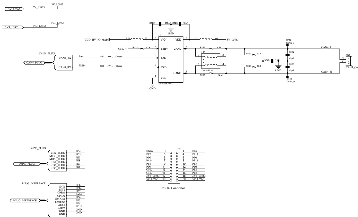
Figure 10. AEK-COM-10BASET circuit schematic (10 of 10)
