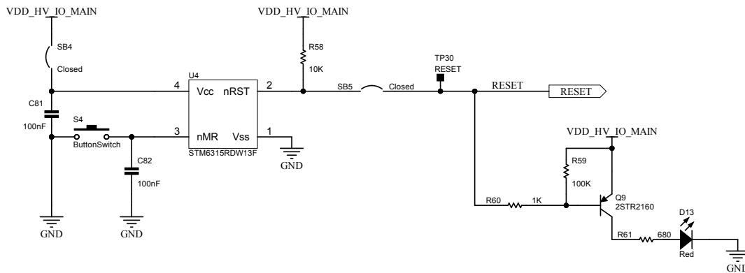
Figure 6. AEK-COM-10BASET circuit schematic (6 of 10)
