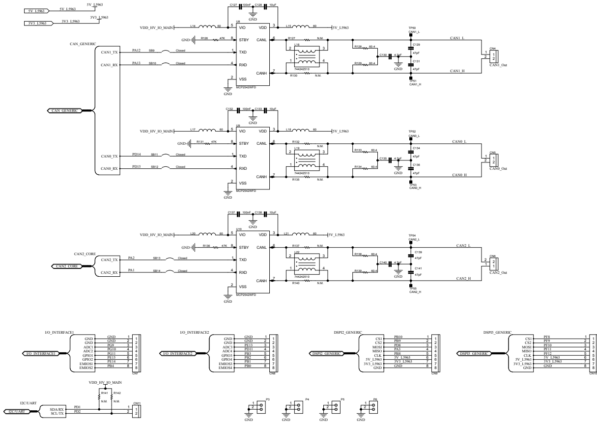
Figure 10. AEK-COM-10BASET circuit schematic (10 of 10)
