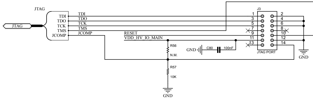
Figure 5. AEK-COM-10BASET circuit schematic (5 of 10)
