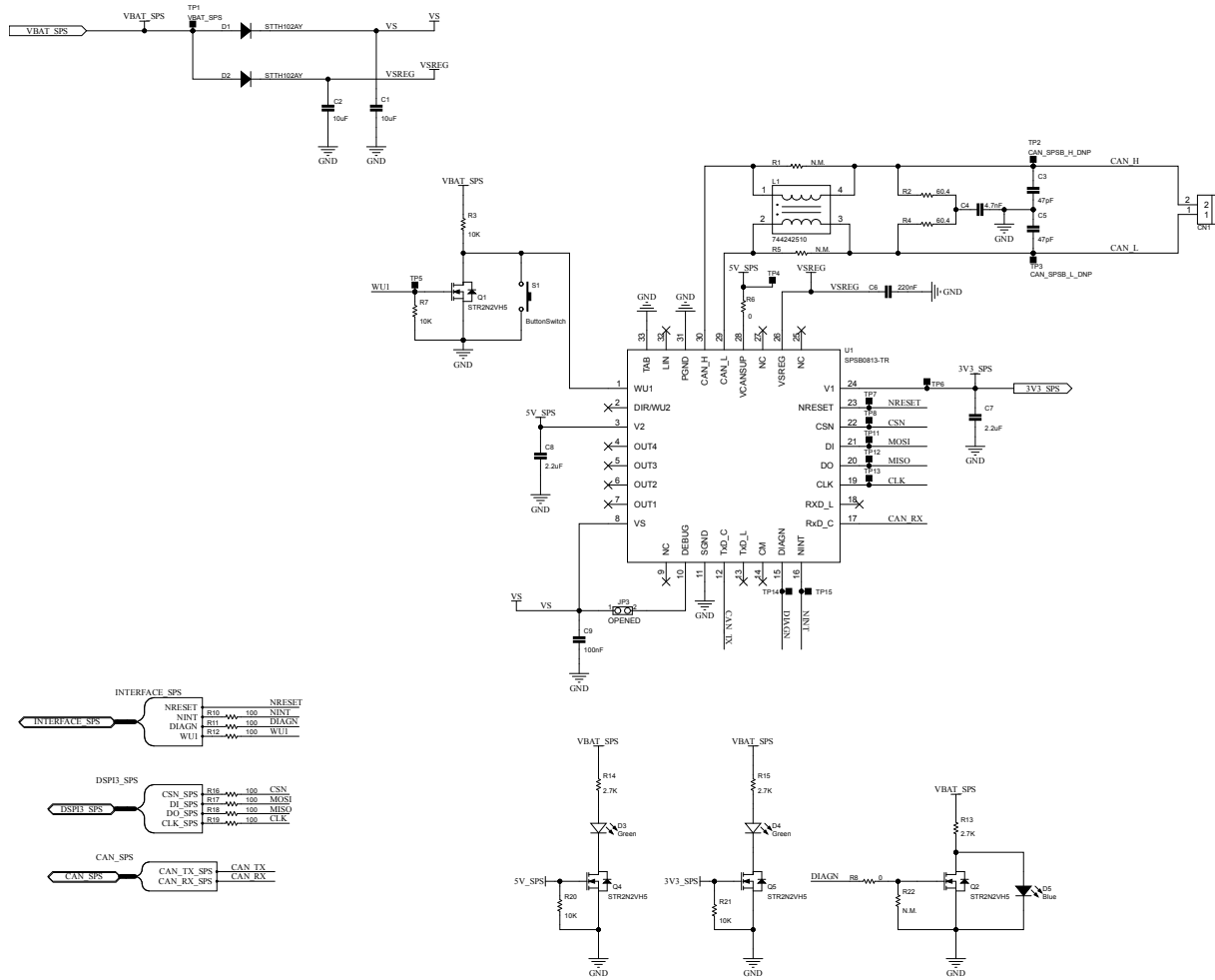
Figure 4. AEK-COM-10BASET circuit schematic (4 of 10)
