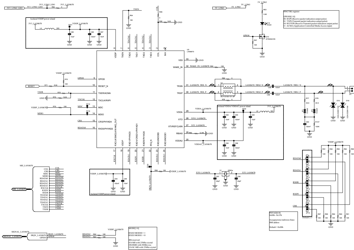
Figure 7. AEK-COM-10BASET circuit schematic (7 of 10)
