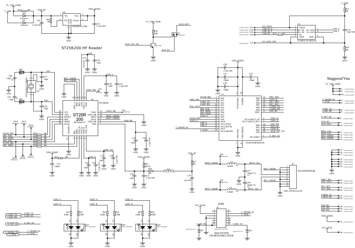
Figure 3. STEVAL-25R200SA main board circuit schematic (3 of 7)
