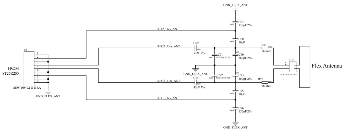
Figure 5. STEVAL-25R200SA main board circuit schematic (5 of 7)
