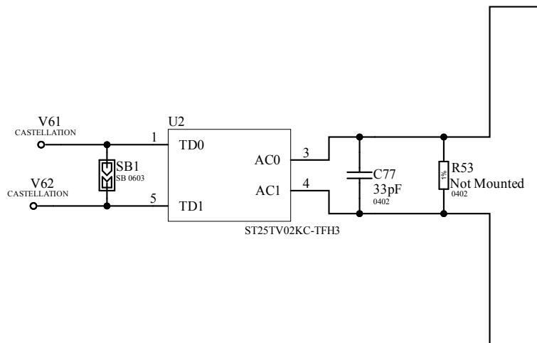
Figure 7. STEVAL-25R200SA main board circuit schematic (7 of 7)
