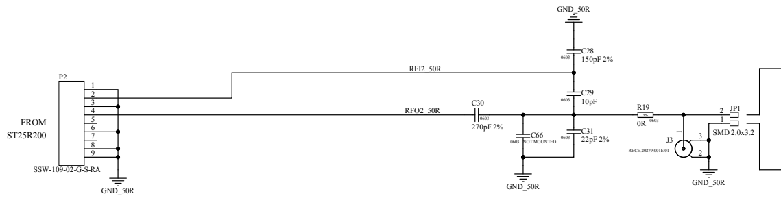
Figure 7. STEVAL-25R200SA main board circuit schematic (7 of 7)
