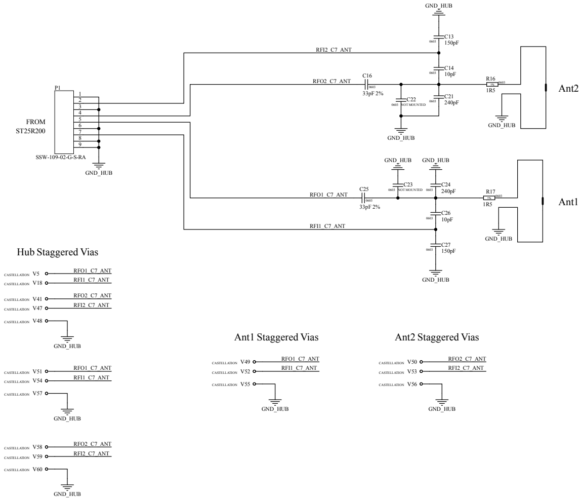
Figure 5. STEVAL-25R200SA main board circuit schematic (5 of 7)
