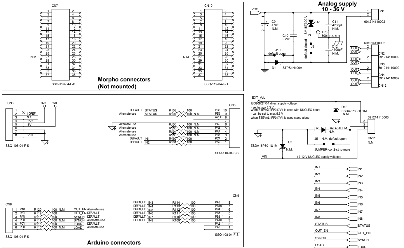
Figure 1. STEVAL-IFP047V1 circuit schematic (1 of 2)
