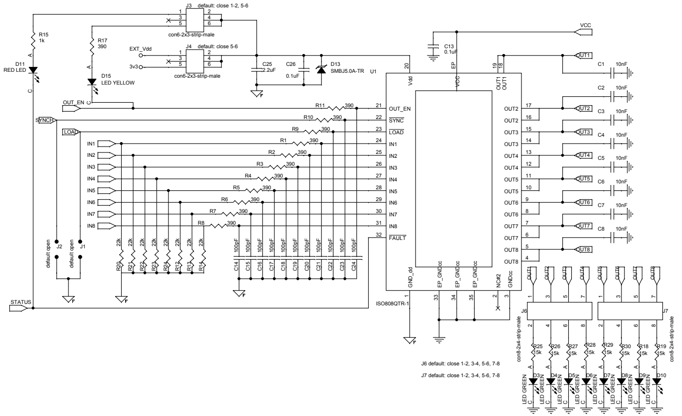
Figure 2. STEVAL-IFP047V1 circuit schematic (2 of 2)
