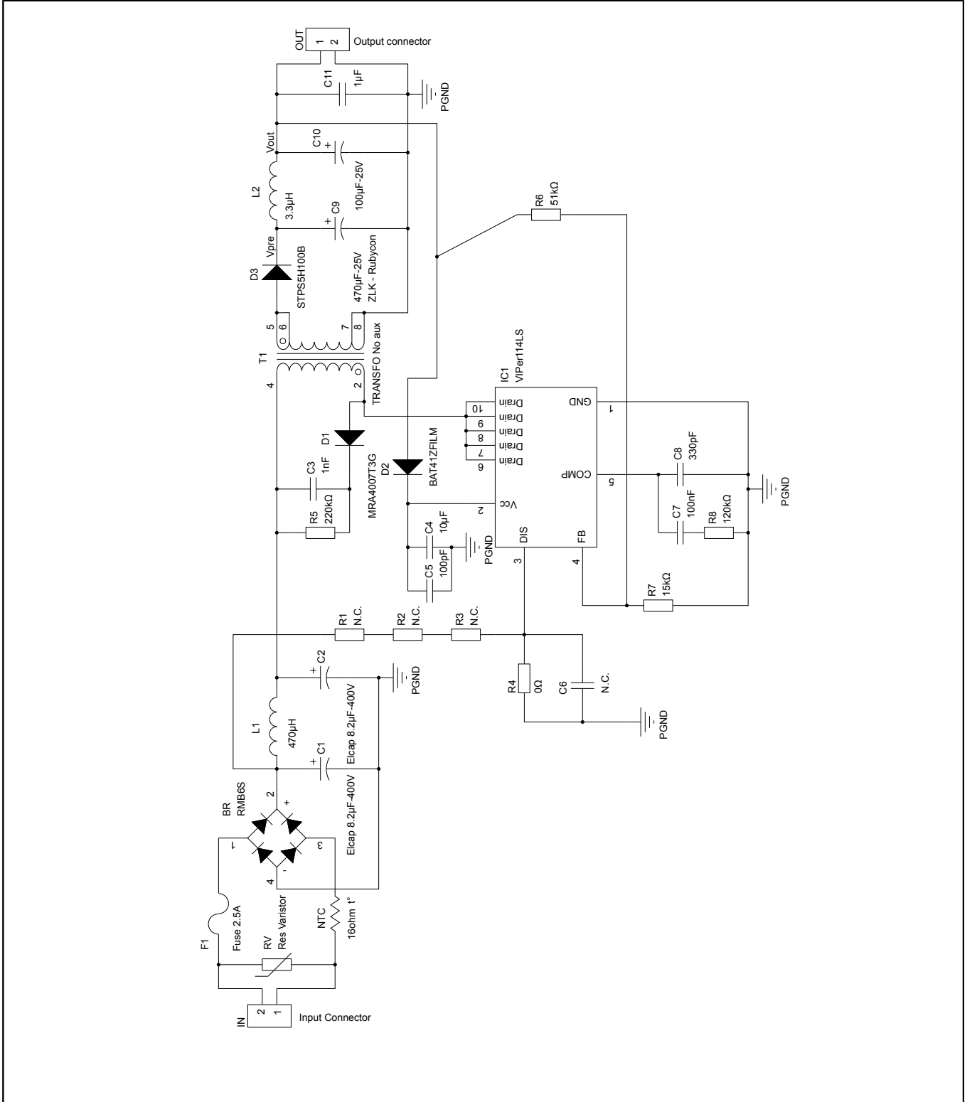
Figure 1: STEVAL-ISA196V1 circuit schematic
