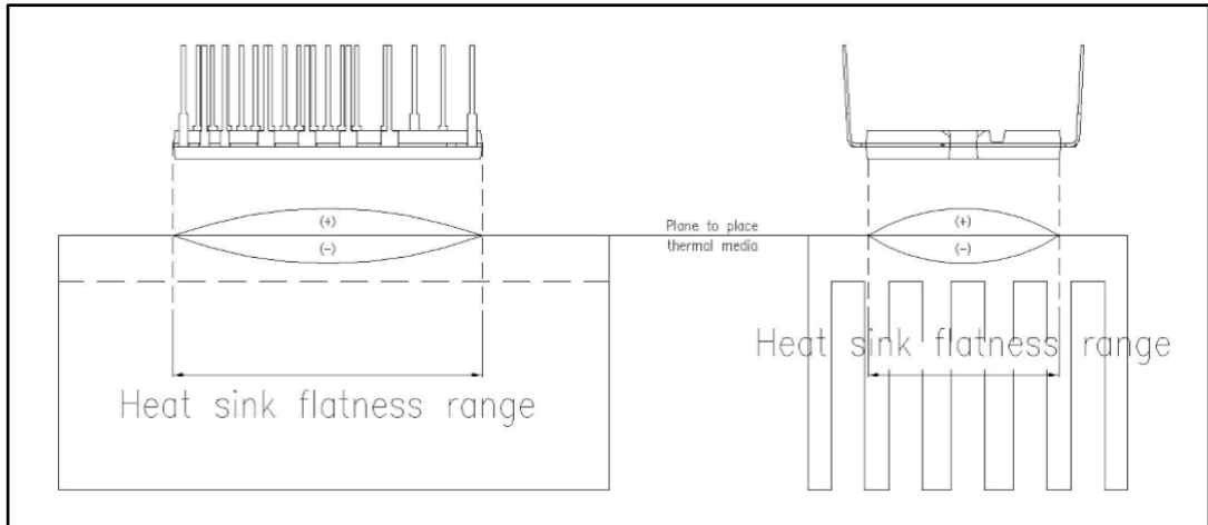
Figure 2: Heat sink flatness specification
