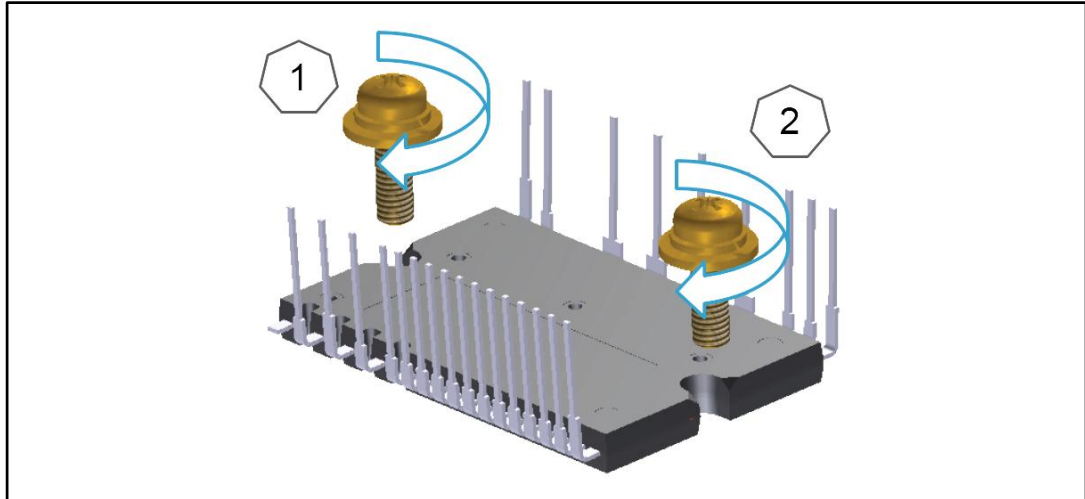
Figure 4: Recommended mounting screw fastening sequence
