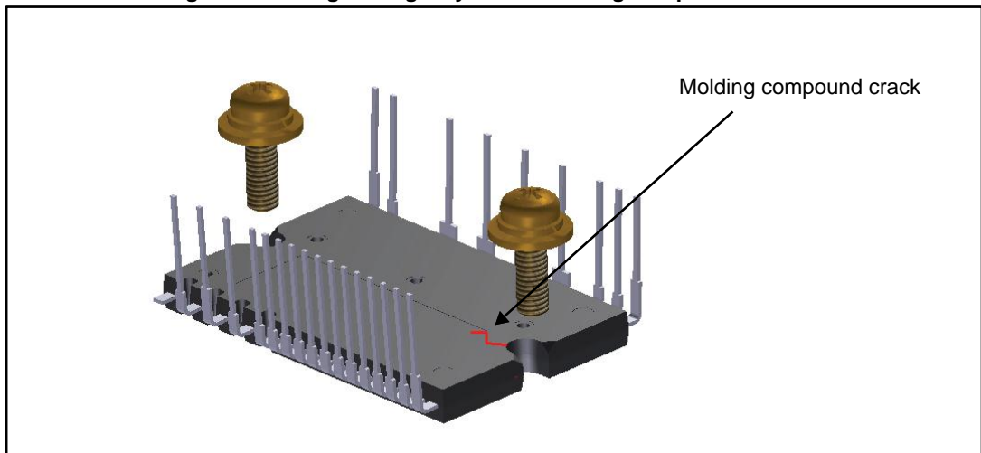
Figure 3: Overtightening may cause molding compound cracks
