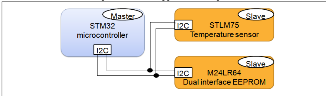
Figure 64. DataLogger block diagram
