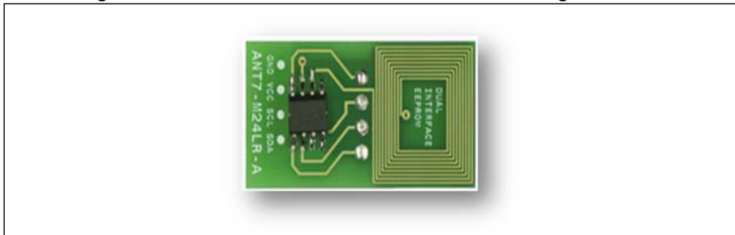
Figure 59. ANT7-M24LR-A dual interface EEPROM daughter board
