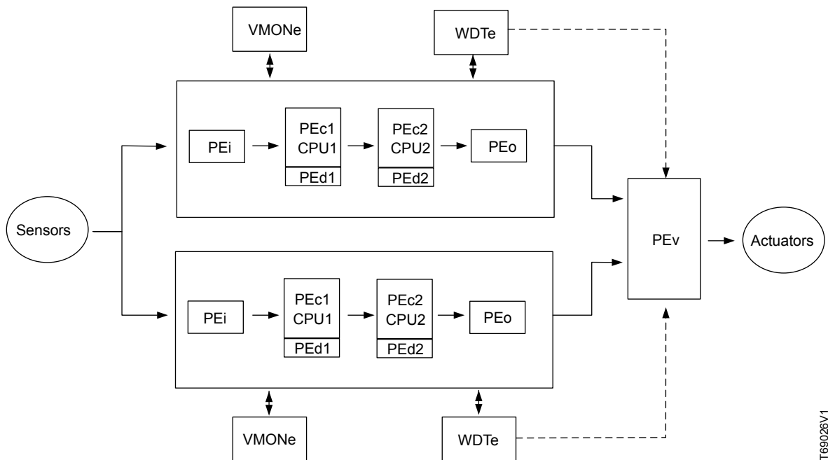
Figure 6. 1oo2 reference architecture
