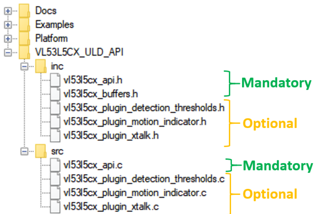
Figure 5. Driver architecture
