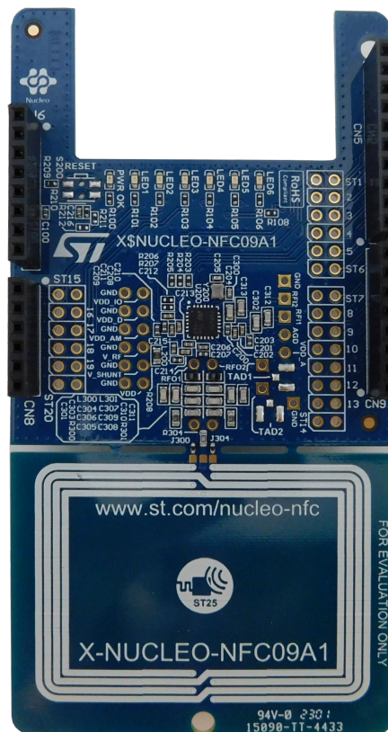
Figure 1. X-NUCLEO-NFC09A1 expansion board
