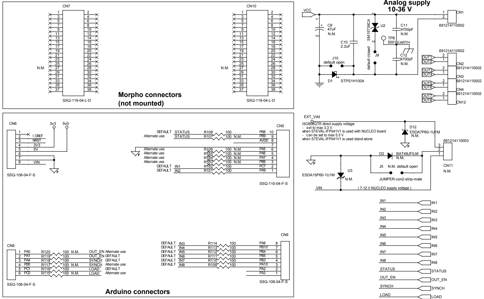
Figure 5. STEVAL-IFP041V1 circuit schematic (1 of 2)
