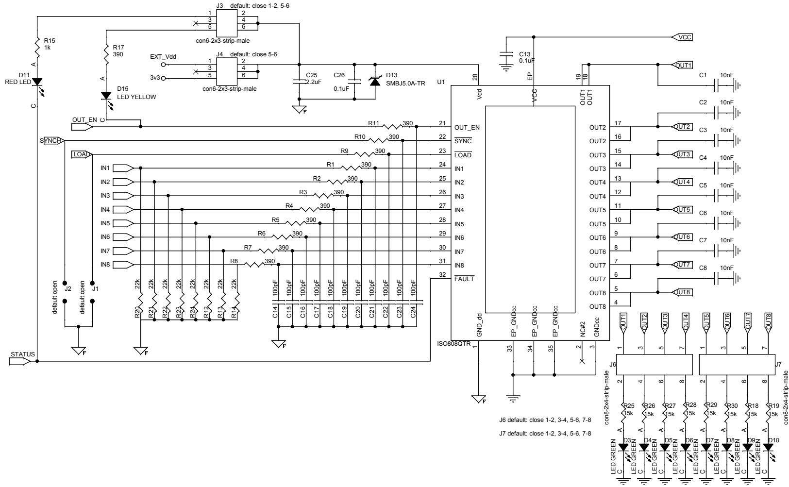
Figure 6. STEVAL-IFP041V1 circuit schematic (2 of 2)
