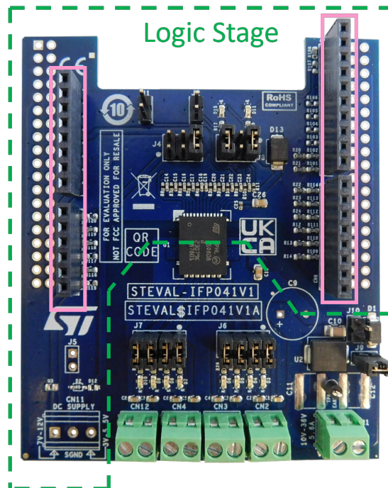
Figure 2. STEVAL-IFP041V1 expansion board: digital interface section
