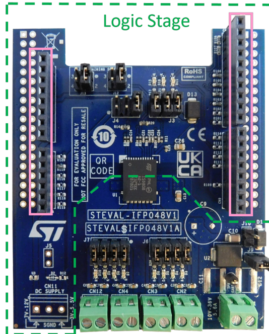
Figure 2. STEVAL-IFP048V1 expansion board: digital interface section
