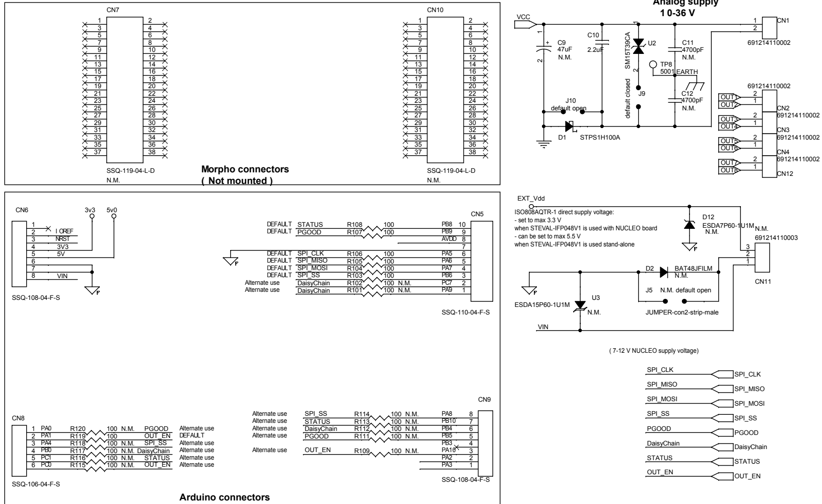
Figure 5. STEVAL-IFP048V1 circuit schematic (1 of 2)
