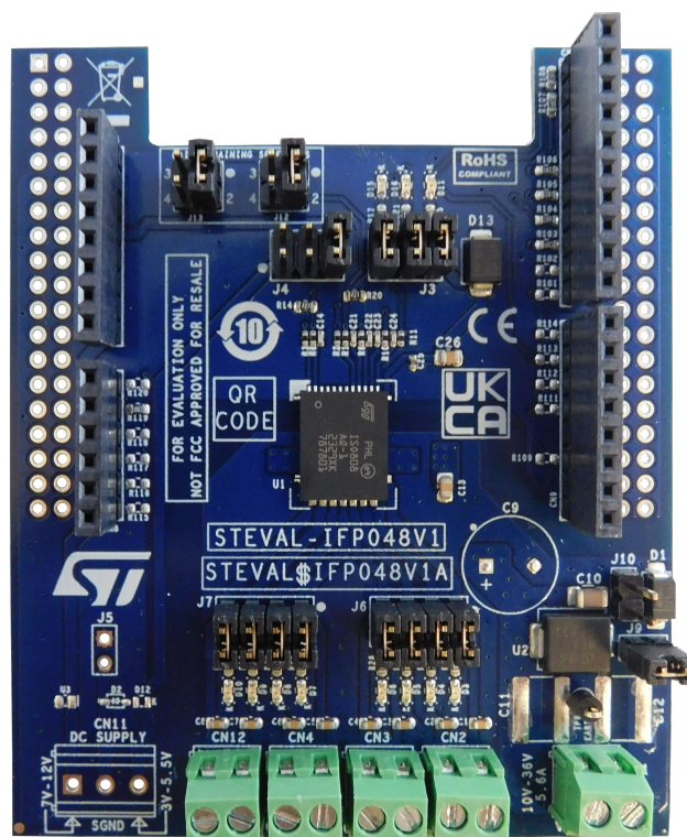
Figure 1. STEVAL-IFP048V1 expansion board
