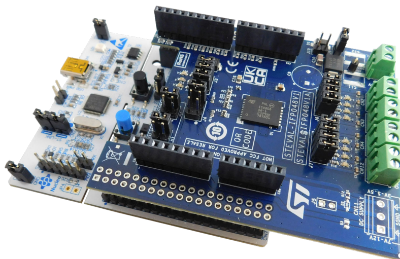
Figure 4. STEVAL-IFP048V1 and STM32 Nucleo stack
