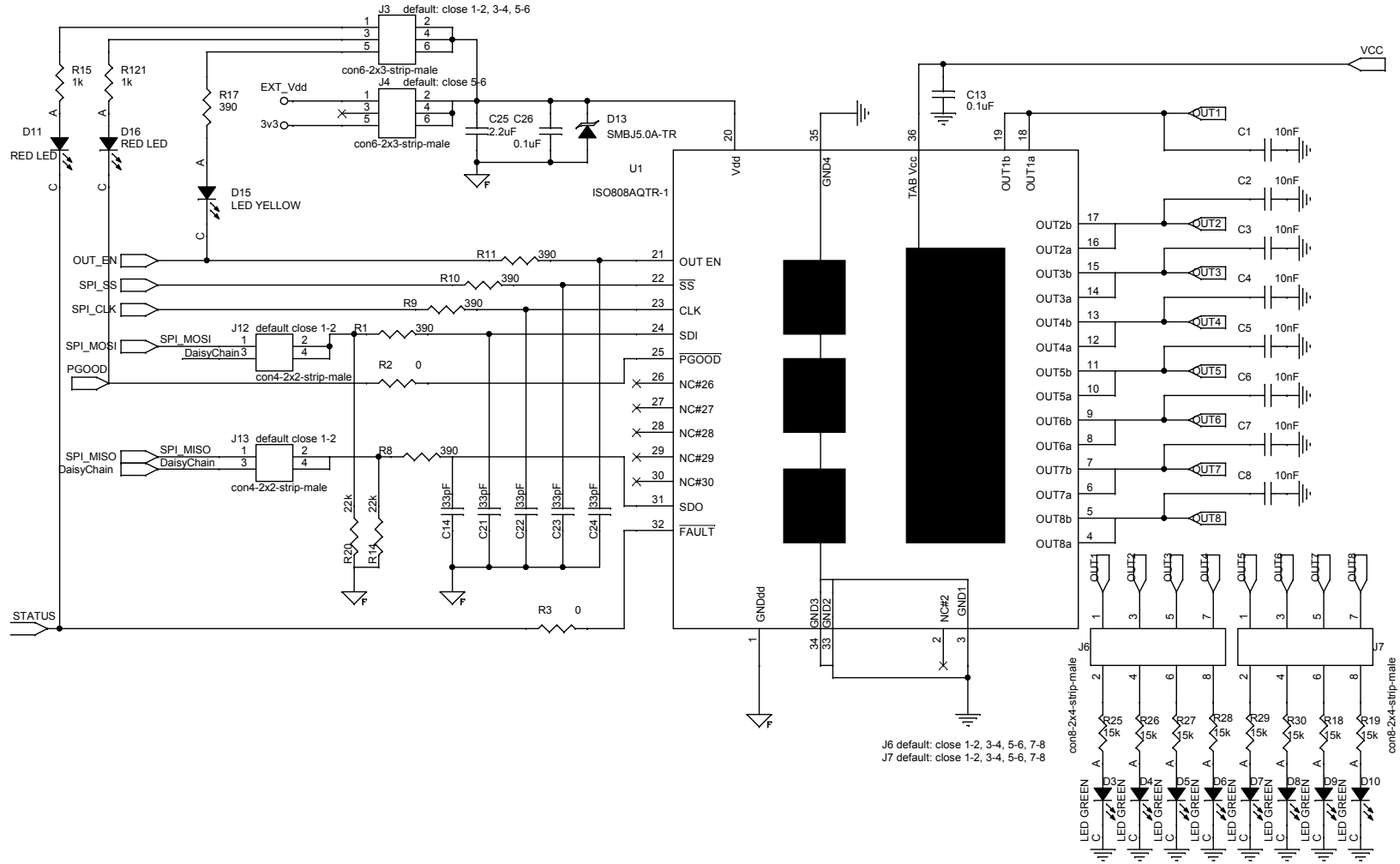
Figure 6. STEVAL-IFP048V1 circuit schematic (2 of 2)
