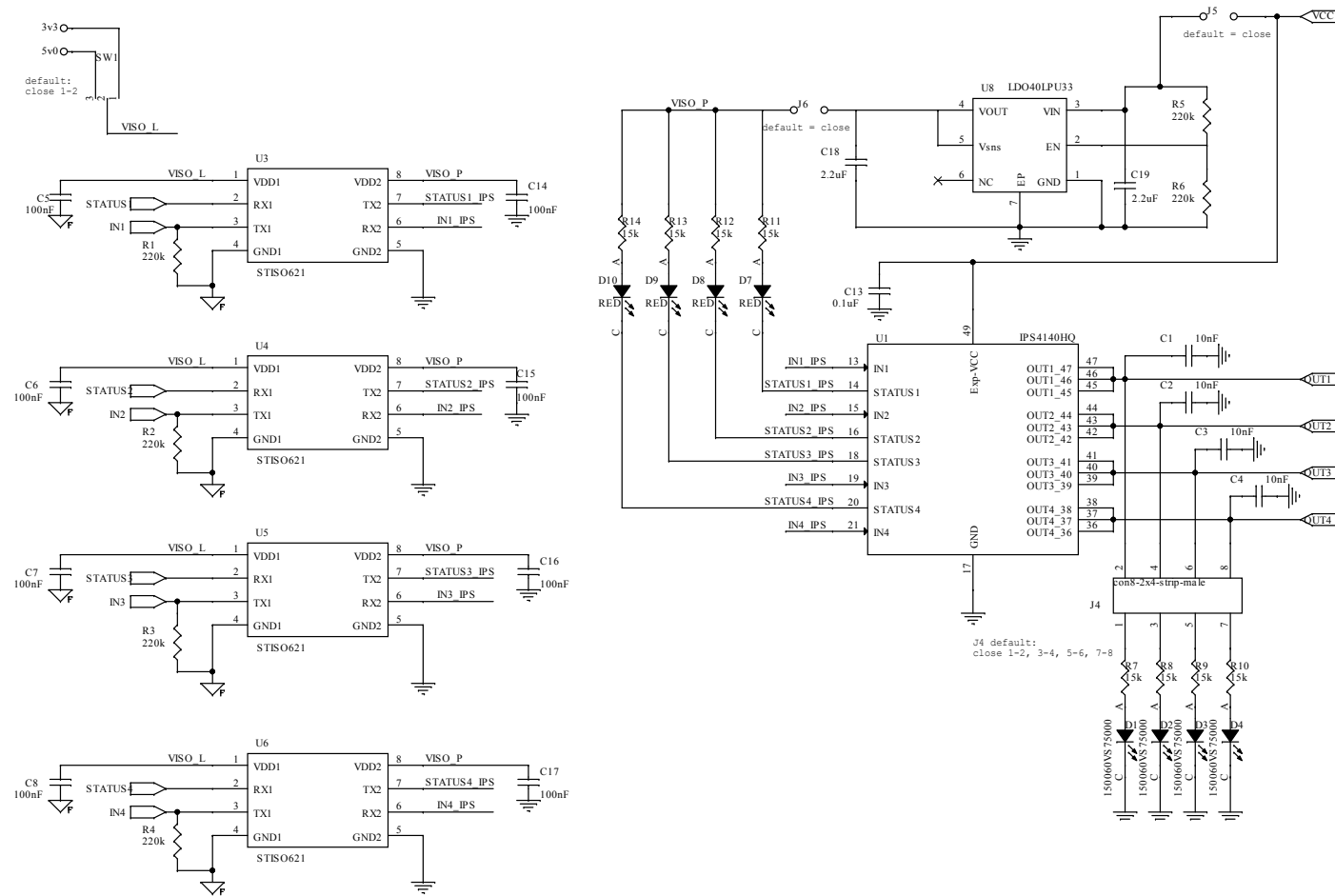
Figure 6. X-NUCLEO-DO40A1 circuit schematic (2 of 2)
