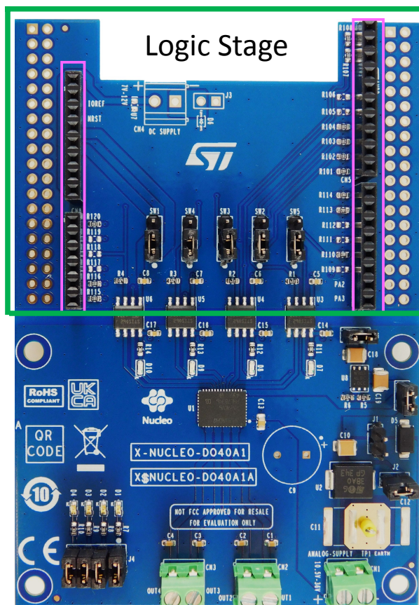
Figure 2. X-NUCLEO-DO40A1 expansion board: digital interface section
