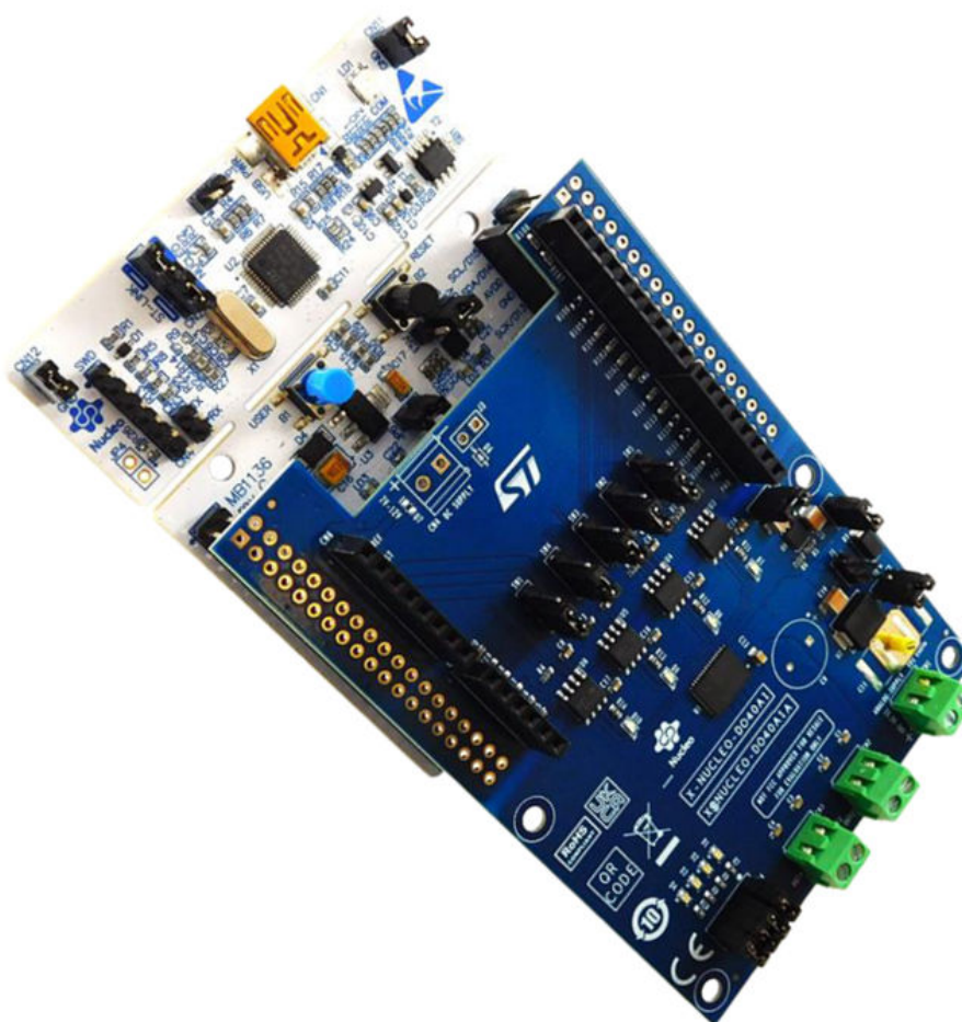
Figure 4. X-NUCLEO-DO40A1 and STM32 Nucleo stack
