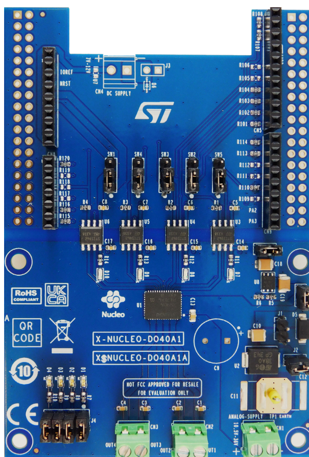
Figure 1. X-NUCLEO-DO40A1 expansion board
