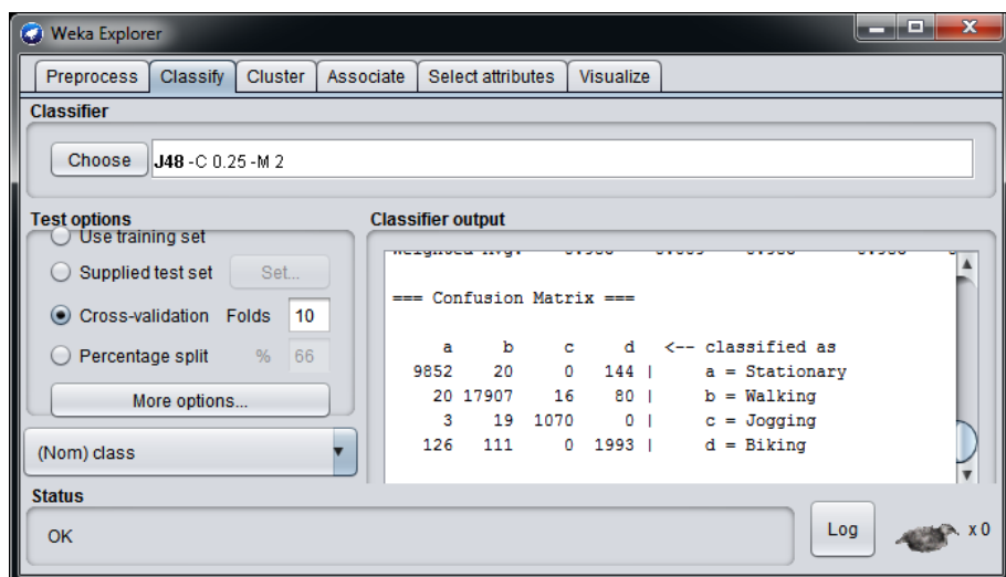
Figure 55. Confusion matrix
