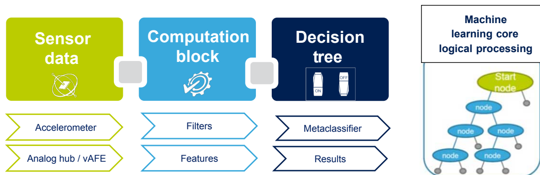
Figure 17. Machine learning core in the ST1VAFE3BX
